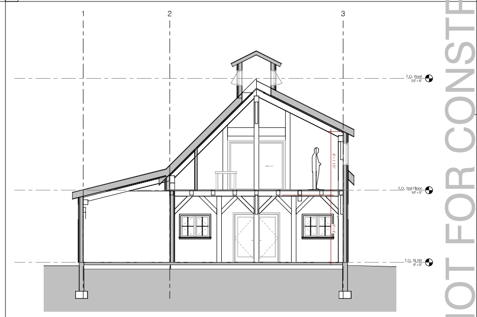
2 Section 2 1/4" = 1'-0"
