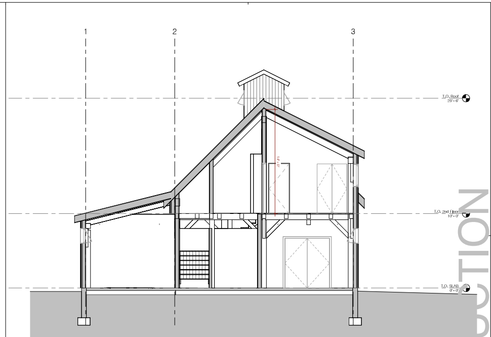
1 Section 1 1/4" = 1'-0"
