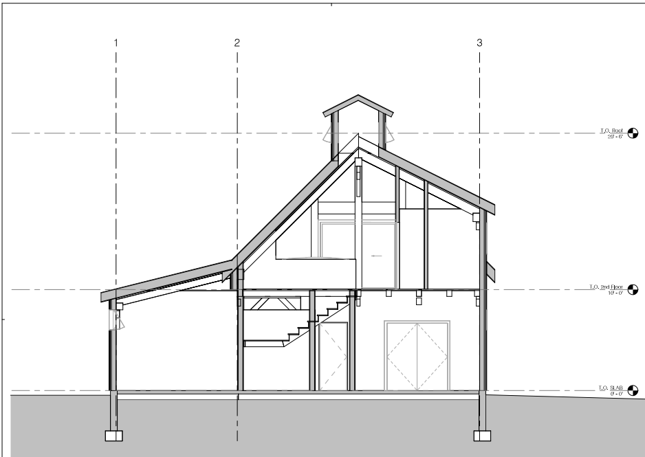
3 Section 3 1/4" = 1'-0"
