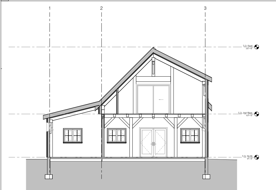
4 Section 4 1/4" = 1'-0"
